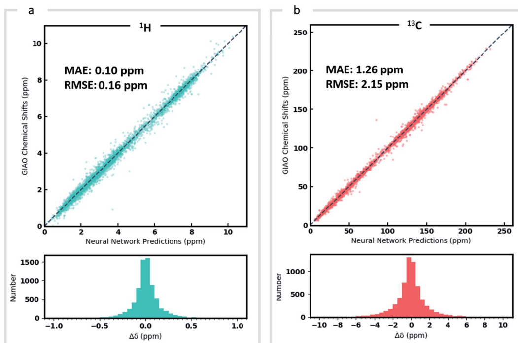
Fig. 2 Prediction of DFT chemical shifts by the trained DFTNN model. Scatter plots and histograms compare DFT computations and GNN predicted chemical shifts for ^1\text{H} (a) and ^{13}\text{C} (b). The held-out test set contains 500 randomly sampled structures (testing/training rate: 1/12) from the DFT8K dataset.
