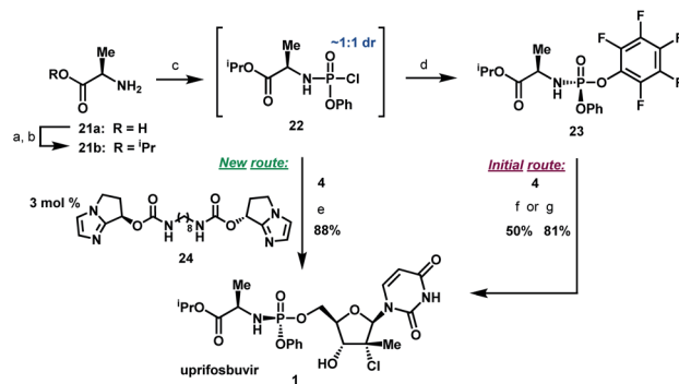
Scheme 6 Completion of uprifosbuvir synthesis. (a) TMS-Cl, i PrOH, 70 °C, 12 h; (b) \text{NEt}_3 , i PrOAc, wiped film evaporation, 80%; (c) \text{PhOP}(\text{O})\text{Cl}_2 , \text{NEt}_3 , i PrOAc, -20 °C, 2 h, 90%; (d) \text{C}_6\text{F}_5\text{OH} , \text{NEt}_3 , i PrOAc, -5 °C to 10 °C, 18 h, 76%; 26 (e) 4 , 3 mol% 24 , 2,6-lutidine, 1,3-dioxolane, -10 °C, 24 h, 88%; (f) 4 , t BuMgCl, THF, -5 °C to 5 °C, 15 h, 50%; 27 (g) 4 , \text{Me}_2\text{AlCl} , 2,6-lutidine, THF, 35 °C, 16 h, 81%. 27
