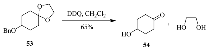
Scheme 24 DDQ-mediated oxidative removal of acetal.
