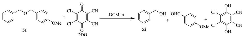
Scheme 23 Deprotection of PMB for hydroxy functionality by DDQ.
