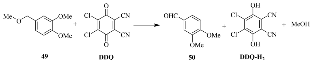
Scheme 22 Cleavage of DMPM protecting group for hydroxy functionality by DDQ oxidation.
