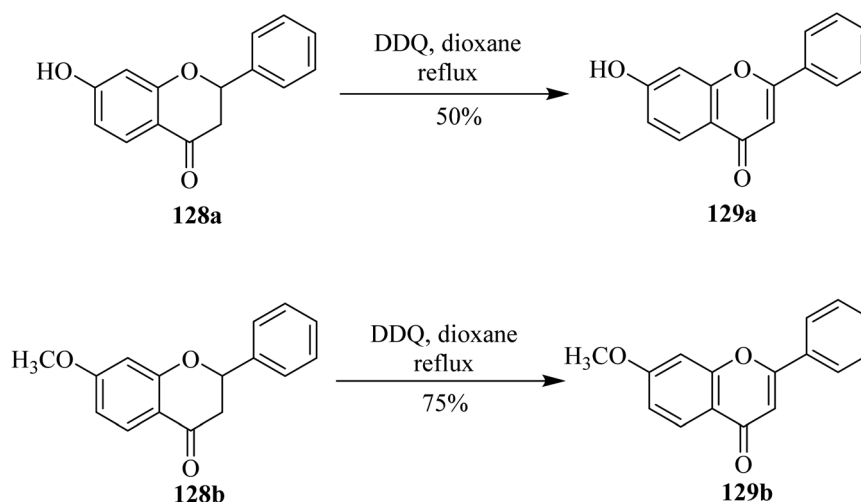
Scheme 46 Dehydrogenation of 7-hydroxyflavanone ( 128a ) and 7-methoxyflavanone ( 128b ).
