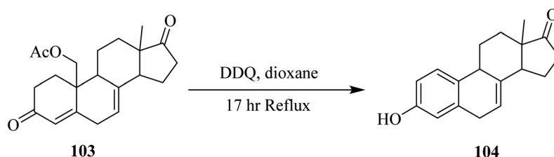
Scheme 41 Dehydrogenation of acetoxy ketones.
