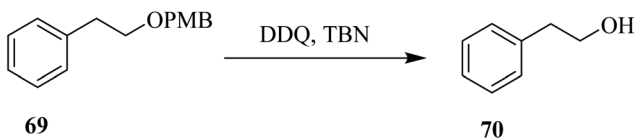
Scheme 30 Deprotection of benzyl-type ethers by DDQ/ tert -butyl nitrite mixture.
