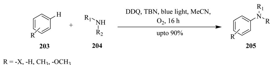
Scheme 71 Amination of aromatic ring via DDQ under visible light irradiation.
