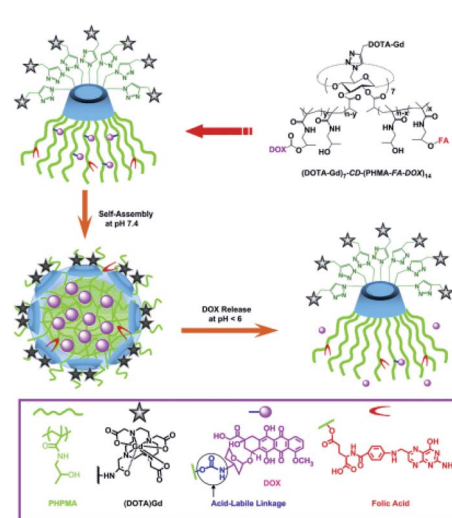
Fig. 35 Fabrication of multifunctional micellar nanoparticles for theranostics based on star copolymers of \beta -CD, (\text{DOTA-Gd})_7\text{-CD-(PHPMA-FA-DOX)}_{14} covalently conjugated with doxorubicin fragments (DOX), folic acid (FA) and DOTA-Gd. The release of DOX is controlled by pH via the cleavage of the carbamate bonds between the DOX and HPMA arms. This figure has been adapted/reproduced from ref. 93 with permission from Elsevier, copyright 2012.
