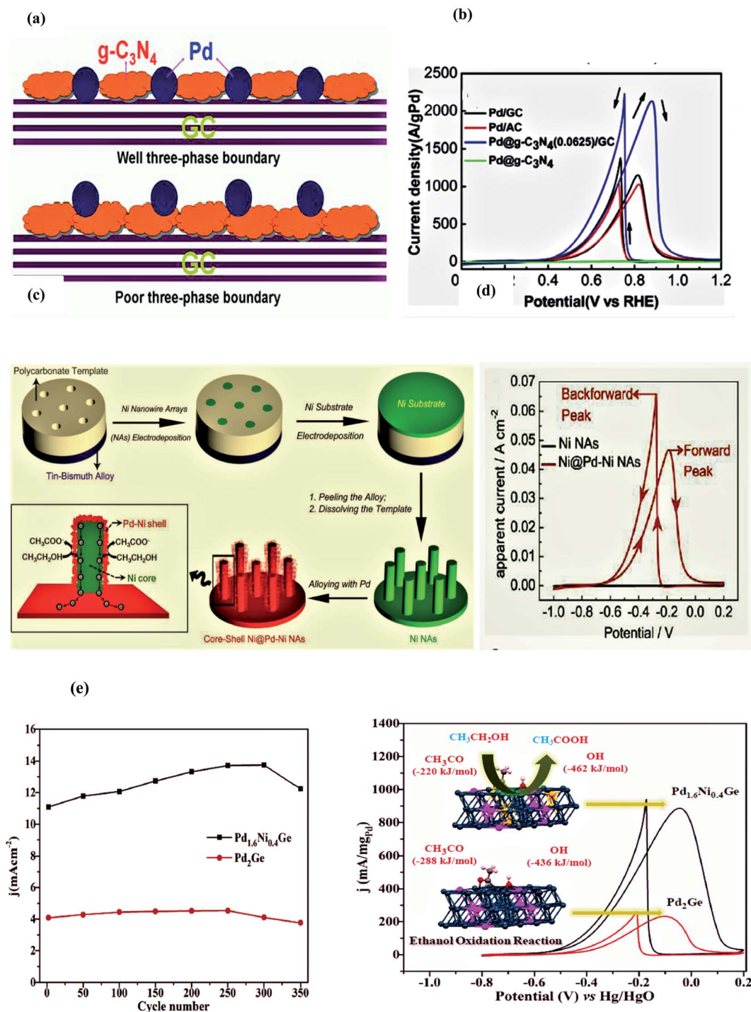
Fig. 6 (a) The development of a three-phase boundary system and (b) CV polarization curves of Pd-based catalysts for the EOR in 1 M KOH and 1 M ethanol solution. Reproduced from ref. 110, Copyright 2016, Elsevier. (c) Synthetic scheme and (b) CV polarization curves of Ni@Pd-Ni nanowire arrays for the EOR in 1 M KOH and 0.5 M ethanol solution. Reproduced from ref. 120, Copyright 2018, ACS. (e) Stability response and CV polarization curves of \text{Pd}_{1.6}\text{Ni}_{0.4}\text{Ge} for the EOR in 1 M KOH and 1 M ethanol solution. Reproduced from ref. 124, Copyright 2019, ACS.
