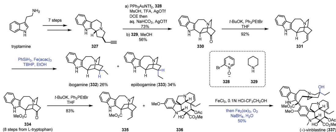
Scheme 41 Luo's synthesis of various iboga alkaloids.
