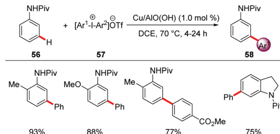
Scheme 19 meta -C–H arylation of anilides 56 with heterogeneous copper nanoparticles.
