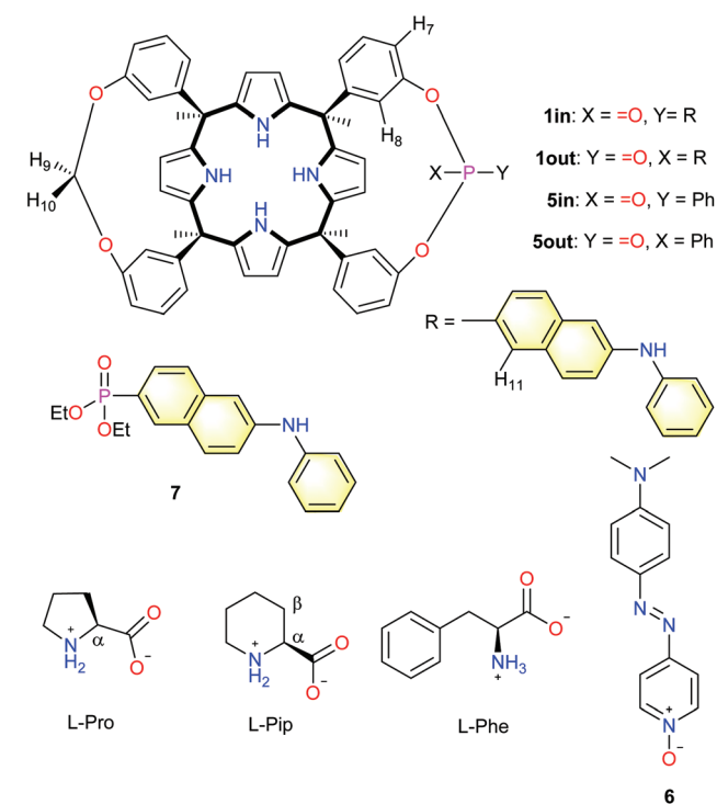
Fig. 1 Line drawing molecular structures of the monophosphonate calix[4]pyrrole cavitands 1in/1out and 5in/5out , the pyridine N -oxide quencher 6 , diethyl 6-(phenylamino)naphthalene-2-phosphonate 7 and the substrates used in the work (L-Pro, L-Pip and L-Phe). Proton assignment of calix[4]pyrrole cavitands and amino acids is shown in the structure.
