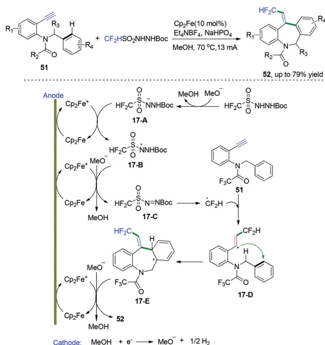
Scheme 26 Electrochemical cascade radical cyclization of alkynes.
