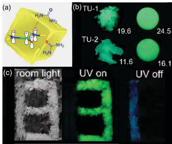
Fig. 25 (a) Structures of urea and TU and their delocalized \pi_s^4 system. (b) Photographs of TU-1, TU-2, and their tablets taken under 312 nm UV light. \phi values (%) of the samples are also given. (c) Pattern "8" comprising urea (blue part) and TU-1 (green part) crystals taken under room light, 312 nm UV light, and after ceasing the UV irradiation. Reprinted with permission from ref. 40. Copyright 2020, John Wiley and Sons.
