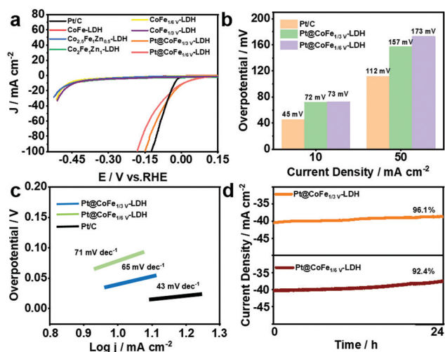
Fig. 4 (a) LSV curves of Pt/C, CoFe-LDH, CoFeZn-LDH, CoFe 1/3 -LDH and Pt@CoFe 1/3 -LDH for catalyzing the HER in 1.0 M KOH. (b) Histogram of the overpotentials of the Pt/C and synthesized nanomaterials to drive 10 mA cm -2 and 50 mA cm -2 . (c) Tafel slopes of Pt/C and Pt@CoFe 1/3 -LDH. (d) Long-term stability measurement of the Pt@CoFe 1/3 -LDH for over 24 h.
