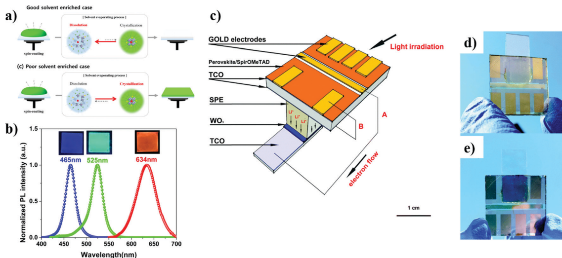
Fig. 11 Perovskite based panchromatic photodetectors and photovoltachromic devices: (a) scheme of the good–poor solvent enriched preparation process of MMH NC films by spin-coating. (b) Normalized PL spectra of blue, green, and red MHP NC-films. Reprinted from Park et al. , Synthesis of post-processable metal halide perovskite nanocrystals via the modified ligand-assisted re-precipitation method and their applications in self-powered panchromatic photodetectors, J. Ind. Eng. Chem. , 92 , 167–173. 148 Copyright 2020, with permission from Elsevier. (c) Scheme of axonometric view of the photovoltachromic device. The optical image of the device under (d) bleached and (e) colored conditions. Reproduced from ref. 149 with permission from The Royal Society of Chemistry.
