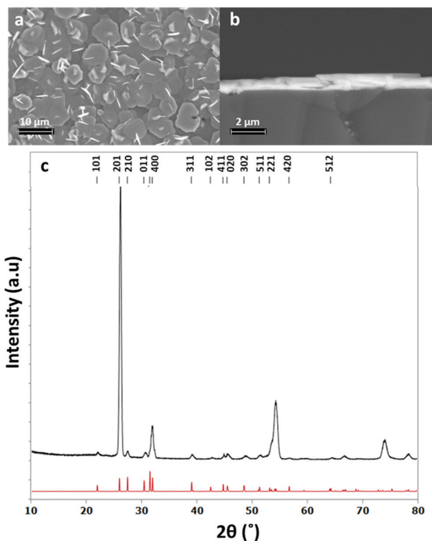
Fig. 4 Top down SEM image (a), cross sectional SEM image (b) and grazing incidence XRD pattern (c) for SnS thin film obtained by low pressure CVD using [\text{Sn}^{\text{n}}\text{Bu}(\text{S}^{\text{n}}\text{Bu})_2] (red = XRD pattern for bulk \text{SnS}^{48} ) with a thickness of around 700 nm.
