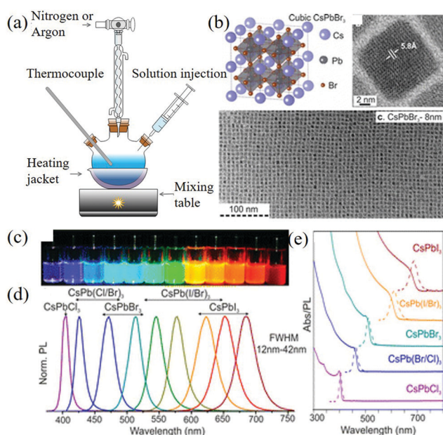
Fig. 3 (a) Colloid quantum dot synthesis device. (b) Schematic of the cubic perovskite lattice and typical transmission electron microscopy (TEM) images of \text{CsPbBr}_3 NCs. (c) \text{CsPbX}_3 NCs ( X = \text{Cl}, \text{Br}, \text{I} ) colloidal solutions in toluene under UV lamp ( \lambda = 365 \text{ nm} ). (d) Representative PL spectra ( \lambda_{\text{exc}} = 400 \text{ nm} for all but 350 \text{ nm} for the \text{CsPbCl}_3 samples). (e) Typical optical absorption and PL spectra (Reproduced from ref. 22 with permission from American Chemical Society).
