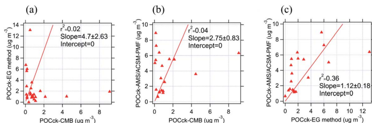
Fig. 5 Correlations of \text{POC}_{\text{ck}} estimated by different methods: (a) extended Gelencs r (EG) method vs. CMB; (b) AMS/ACSM-PMF vs. CMB; (c) AMS/ACSM-PMF vs. EG method.
