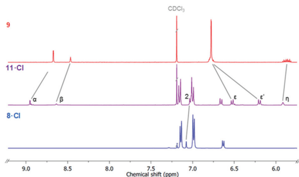
Fig. 2 Stacked truncated ^1\text{H} NMR spectra of macrocycle precursors 9 (top), XB [2] rotaxane 11-Cl (middle) and free axle 8-Cl ( \text{CDCl}_3 , 500 MHz, 298 K).
