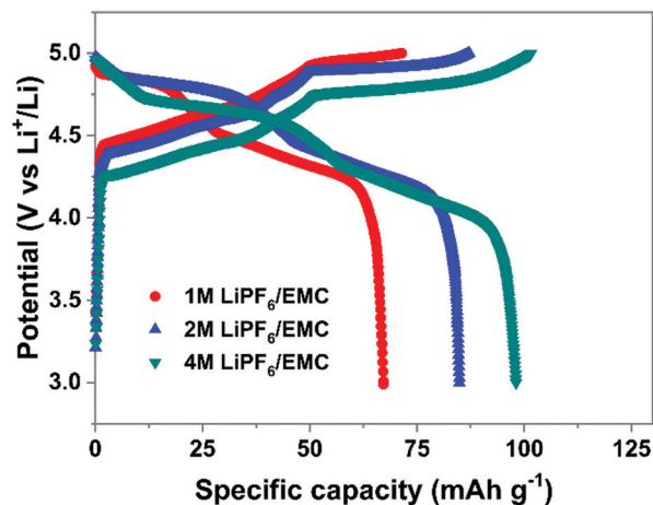
Fig. 11 Charge–discharge profiles of the graphite cathode in different concentration electrolytes. Li//graphite half cells were used. Electrolytes are 1–4 M LiPF 6 in EMC. The current density is 100 mA g -1 .
