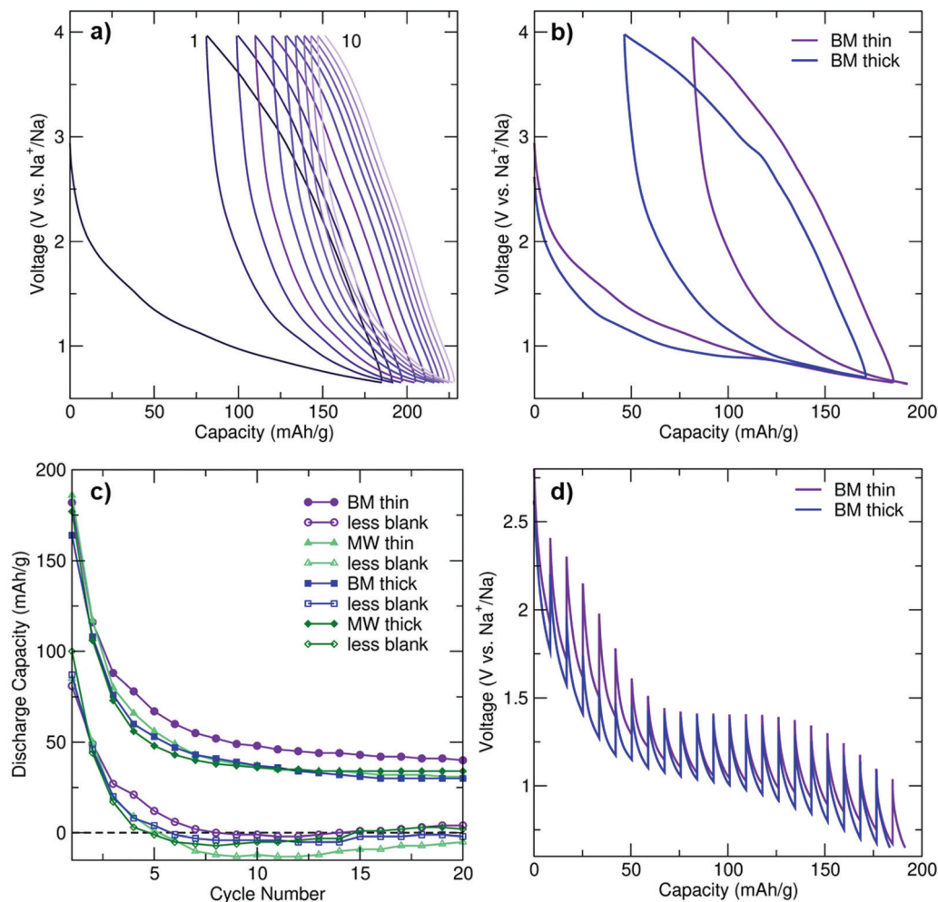
Fig. 2 Electrochemical characterization of \text{Na}_3\text{FeF}_6 . (a) First ten cycles for \text{BM-Na}_3\text{FeF}_6 thin cells (C/20 rate). (b) First two charge and discharge cycles for \text{BM-Na}_3\text{FeF}_6 thin and thick cells (C/20 rate). (c) Discharge capacity retention for \text{Na}_3\text{FeF}_6 cells (filled symbols) and for \text{Na}_3\text{FeF}_6 cells with the corresponding blank cell capacity subtracted (unfilled symbols). Three cells were averaged for each point. (d) GITT test (C/20 rate) for the first discharge cycle of \text{BM} thin and thick cells.
