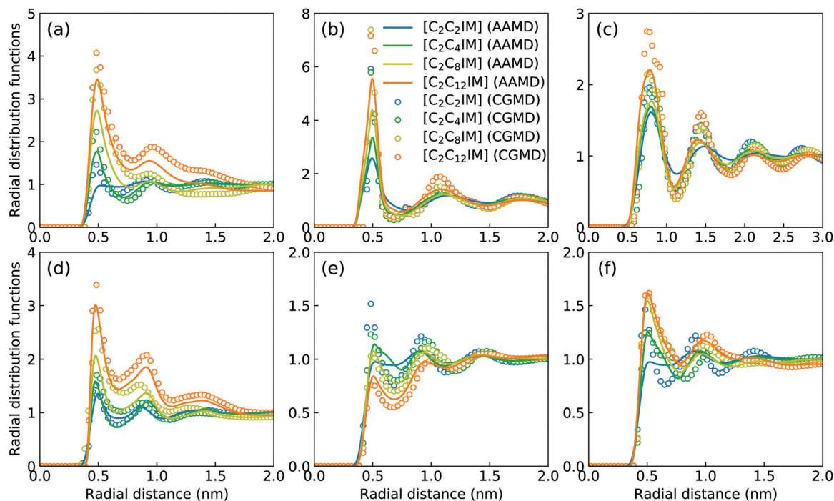
Fig. 3 Representative radial distribution functions of (a) IM–IM, (b) IM–BF, (c) BF–BF, (d) CH–CH, (e) CH–CE(CT), and (f) CE(CT)–CE(CT) pairs for [C_{2C_n}IM][BF_4] ILs obtained from reference AA and CG MD simulations performed at 400 K.
