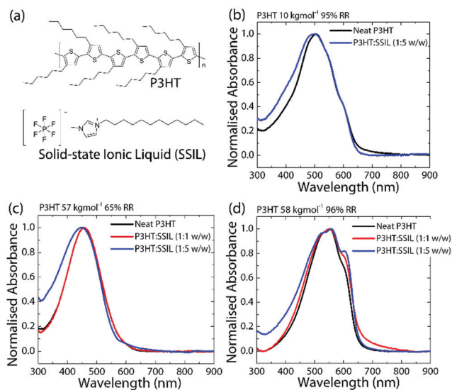
Fig. 1 (a) Chemical structure of the conjugated polymer P3HT and the solid state ionic liquid [C 12 H 25 IM + ][PF 6 - ] (SSIL). Normalised absorbance spectra of P3HT neat, 1:1 and 1:5 for (b) low M_w and high RR, (c) high M_w and low RR and (d) high M_w and RR P3HT blends.
