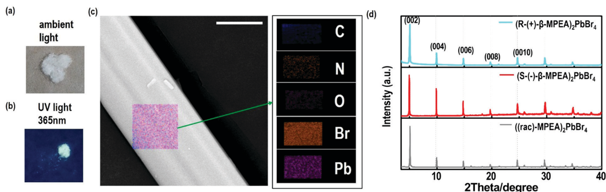
Fig. 1 The optical image under (a) ambient light and (b) UV light (365 nm), (c) SEM image (scale bar is 5 μm) and element mapping images of ( R -(+)- \beta -MPEA) 2 PbBr 4 . (d) The XRD patterns of perovskite crystals.
