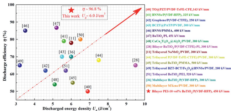
Fig. 6 Comparison of energy density and efficiency of this work (PEI-10 vol% \text{BaTiO}_3/\text{P}(\text{VDF-HFP}) composite) and reported results.
