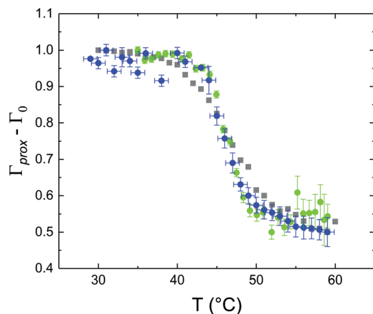
Fig. 4 Temperature dependence of \Gamma_{\text{prox}} - \Gamma_0 obtained from the analysis of TTR-NR data for the fast (blue circles) and slow (green dots) temperature scans. The temperature evolution of the \Gamma_{\text{prox}} parameter obtained from a Monte Carlo simulation for the LFF in an asymmetric SLB is plotted with gray squares for comparison purposes. Since the slow scan included constant temperature steps, the average value of \Gamma_{\text{prox}} - \Gamma_0 is reported for each temperature. For all datasets, to account for initial compositional differences (in terms of ratio between deuterated and protiated lipids), \Gamma_0 (initial level of mixing) was subtracted from \Gamma_{\text{prox}} .
