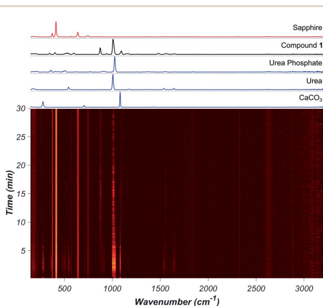
Fig. 2 (Bottom) In situ Raman spectra of the neat milling reaction between \text{CaCO}_3 , urea, and urea phosphate. Brighter colour denotes higher intensity. (Top) Raman spectra of reactants (blue), the product (black), and background from the sapphire milling jar (red) with individual spectra of reactants and product above the 2D plot.
