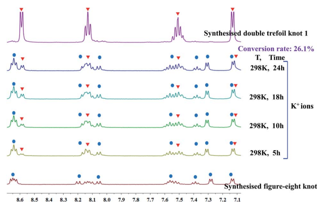
Fig. 4 Partial ^1\text{H} NMR spectra ( \text{CD}_3\text{OD} , 400 MHz, 298 K) concerning structural unlinking transformation of figure-eight knot to double trefoil knot 1 induced by \text{K}^+ ions. Blue circles denote signals of figure-eight knot; red triangles denote double signals of the trefoil knots.
