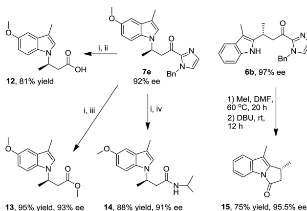
Scheme 2 Synthetic elaboration studies. Reaction conditions: (i) MeI, DMF, 60 °C, 20 h; (ii) DBU, H 2 O, rt, 4 h; (iii) DBU, CH 3 OH, CH 2 Cl 2 , rt, 6 h; (iv) DBU, t PrNH 2 , rt, 12 h.
