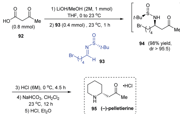
Scheme 17 Synthesis of (-)-pelletierine commencing from sulfonimine 93 .
