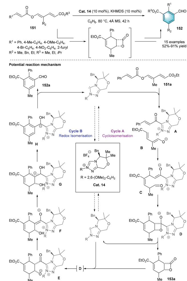
Scheme 44 NHC-catalyzed intramolecular benzannulation to synthesize tri-substituted benzaldehydes.
