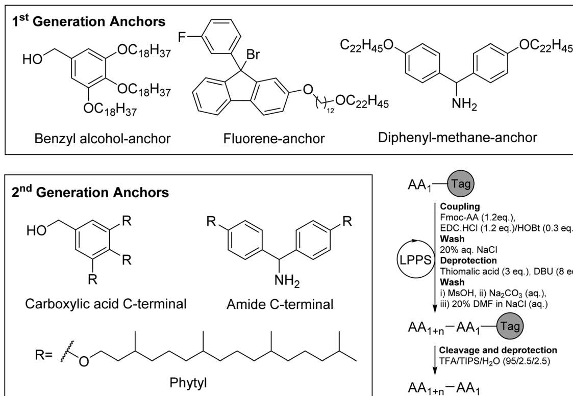
Fig. 8 Ajjiphase® soluble anchors for liquid-phase peptide synthesis (LPPS) developed by Takahashi et al. and commercialised by Ajinomoto Bio-Pharma Services. 105–107
