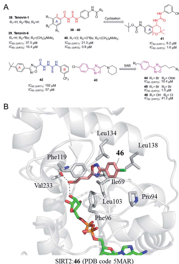
Fig. 7 (A) Chemical structures of Tenovins and oxadiazoles-based SIRT2 inhibitors and their inhibitory activity data on SIRTs determined by coupled enzymatic deacetylation assay. 55 (B) Crystallographic analyses revealed the binding features of 46 with SIRT2. 55
