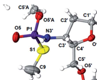
Fig. 1 Crystal structure of DMT-dG^{iBu}_{NPSMe}T_{OAc} 10f showing partial structure and spatial orientation of substituents around the phosphorus stereogenic center (marked P1). Compound 10 was obtained from the monomer 6Gf (fast-eluting 5'- O -DMT-3'-amino-2',3'-dideoxy- N6 - iBu -guanosine-3'- N -(2-thio-4,4-pentamethylene-1,3,2-oxathiaphospholane). The oxygen atom marked O5'A belongs to the thymidine residue.
