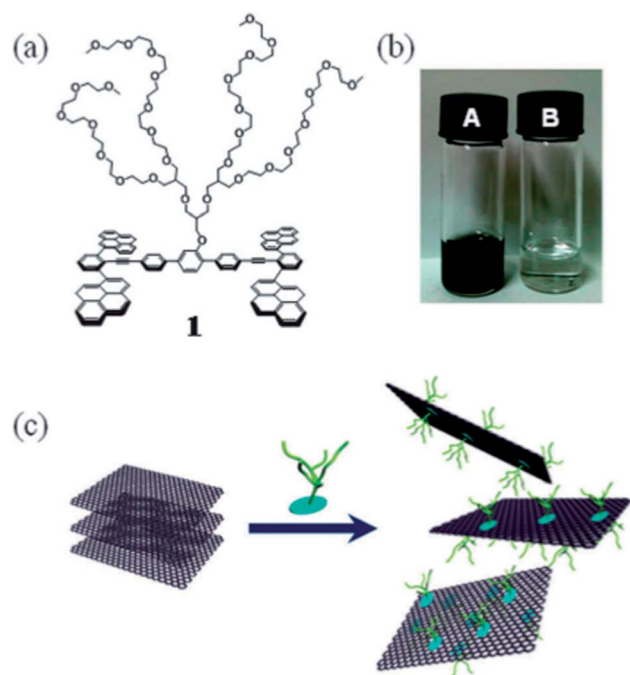
Fig. 13 Exfoliation process of graphite and stabilization of graphene through the \pi - \pi interaction with tetraterpene derivative. This figure has been reproduced from ref. 91 with permission from R. Soc. Chem. , Copyright 2016.
