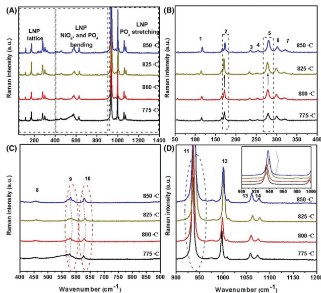
Fig. 22 (A) The Raman spectra of LNP ceramics; (B) the modes in 50–400 \text{cm}^{-1} representing the lattice modes; (C) the modes in 400–900 \text{cm}^{-1} representing mainly symmetric and antisymmetric bending modes of O–P–O and Ni–O; (D) the modes in 900–1200 \text{cm}^{-1} representing the symmetric and asymmetric stretching mode vibrations of the [\text{PO}_4]^{3-} anion (reprinted with permission from ref. 173. Copyright 2019 John Wiley and Sons).
