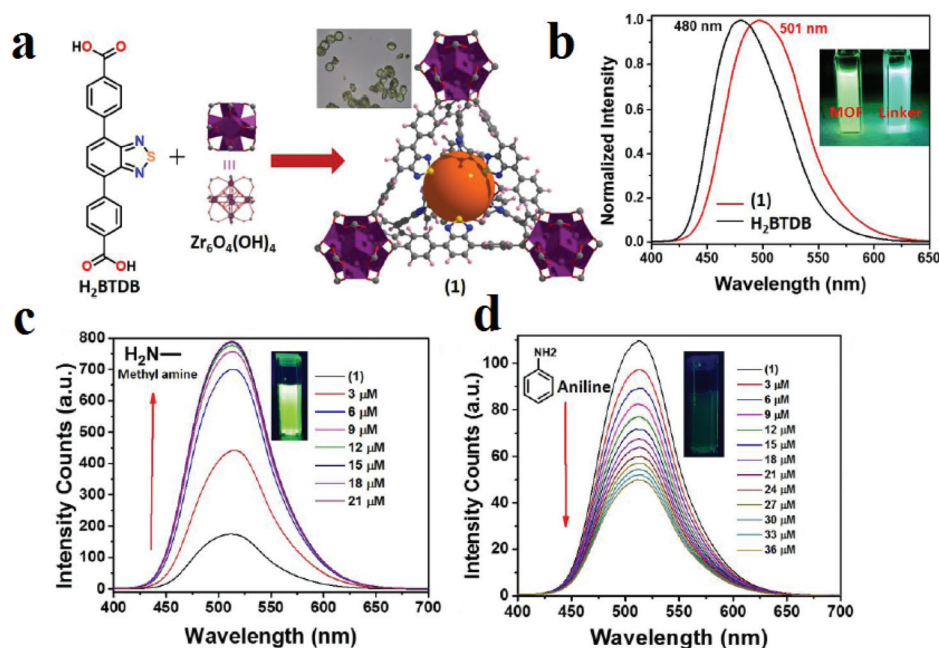
Fig. 23 Application of Zr-BTDB-fcu-MOF in amine detection. (a) Schematic of the synthesis of Zr-BTDB-fcu-MOF. (b) PL spectra of the MOF (red) and linker (black). Fluorescence intensities of MOF aqueous suspension upon addition of 3 \mu M increments of methylamine (c) and aniline (d) ( \lambda_{\text{max}} = 515 nm). Reproduced with permission from ref. 432.
