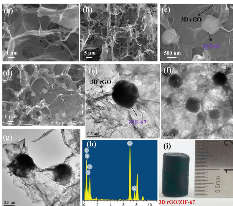
Fig. 9 The SEM images of (a and b) 3D rGO aerogel and (c and d) 3D rGO/ZIF-67 aerogel, and the TEM (e, f and g), (h) EDX and (i) digital photographs of the 3D rGO/ZIF-67 aerogel. Reprinted with permission from ref. 132. Copyright 2018 Elsevier.
