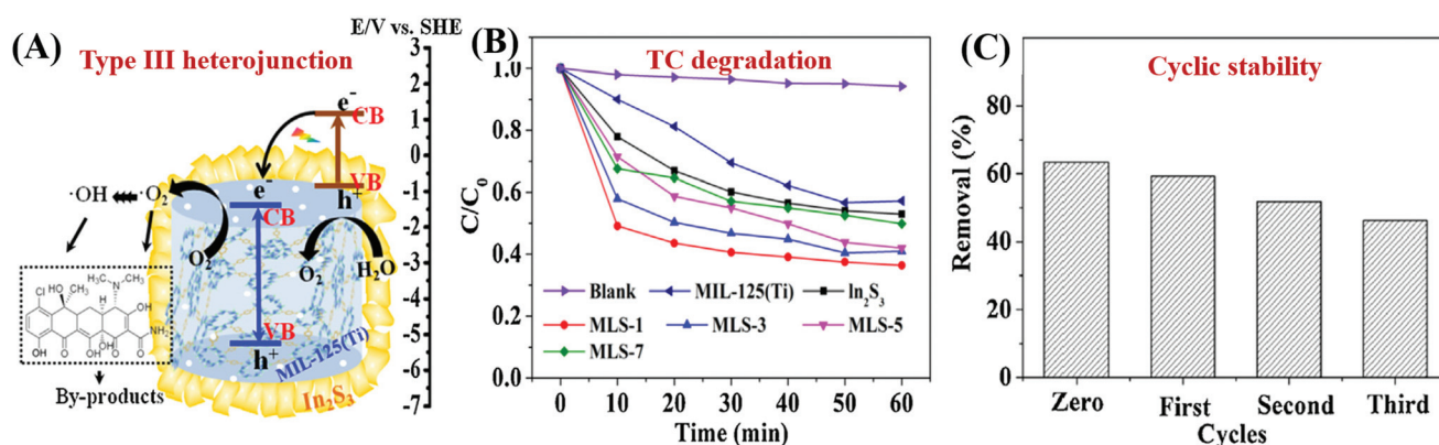
Fig. 29 (A) Proposed mechanism for the charge transfer processes in In_2S_3 @MIL-125(Ti); (B) photocatalytic degradation of TC by different samples; (C) cycling stability of optimized In_2S_3 @MIL-125(Ti) for TC degradation under visible light. Adapted with permission from ref. 204, © 2016 Elsevier.
