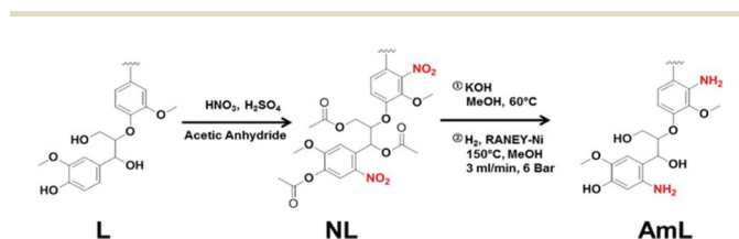
Fig. 2 Synthetic pathway for the conversion of alkali-lignin (L) into aminated lignin (AmL) via aromatic nitration.
