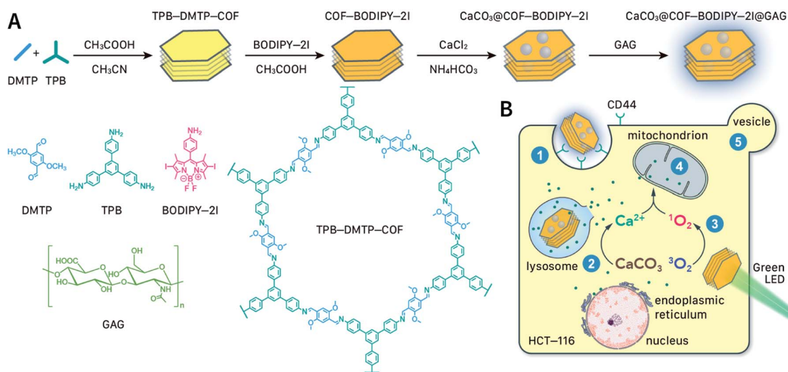
Fig. 81 COF-based composite nanomaterial for synergistic \text{Ca}^{2+} overload and PDT. (A) Synthesis of \text{CaCO}_3@ \text{COF-BODIPY-2I@GAG} . (B) Schematic illustration of combination therapy under green LED irradiation. (1) CD44-mediated cellular uptake; (2) \text{CaCO}_3 decomposition in lysosomes; (3) ^1\text{O}_2 generation induced by BODIPY-2I PS under green LED; (4) damaged mitochondrial function co-induced by ^1\text{O}_2 and \text{Ca}^{2+} ; (5) tumor cell blebbing due to oncosis. Adapted with permission. 415 Copyright 2020, Wiley-VCH Verlag GmbH & Co. KGaA, Weinheim.
