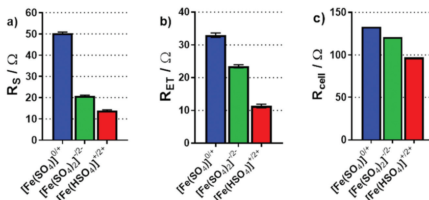
Fig. 8 Bar charts summarising (a) the solution resistance, R_s and (b) the electron transfer resistance, R_{ET} , determined through impedance spectroscopy in the non-isothermal thermocell. Also shown is (c) the calculated total thermocell resistance, R_{cell} of the thermogalvanic cell during steady-state discharge, based upon Ohm's Law ( V = IR ) from I - V plots during power production. All measurements were taken at an applied \Delta T of 20 \text{ K} ( T_c = 20^\circ \text{C} ). For EIS analysis, the spectra are included in the ESI,† and the fitting model has been previously reported elsewhere. 22
