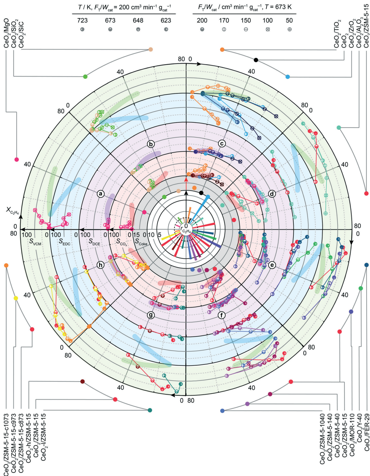
Fig. 3 Reaction rates (in mol h -1 mol Ce -1 ) and coke selectivity (in %) at 673 K, and product selectivities (in %) recorded as a function of ethene conversion (in %) for ceria catalysts supported over a)–d) different carriers, and e)–h) zeolite supports, with various framework types, Si:Al ratios, Ce-loading, and calcination temperatures, respectively. The catalysts are identified by a colour code, indicated on the outside of the circle, while catalytic data points were recorded using the conditions that are specified by the symbol interior, as indicated at the top. The performance of bulk CeO 2 is used as a benchmark, indicated by the dashed circle and highlighted regions. Conditions are detailed in Table 2.
