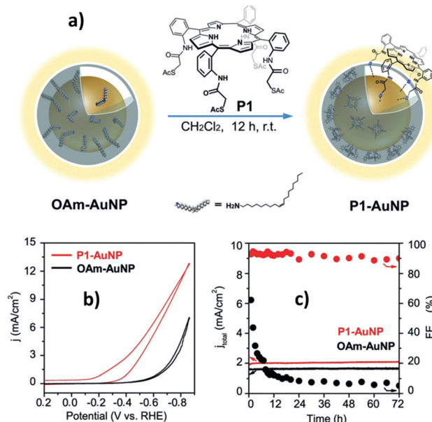
Fig. 32 (a) Synthesis of P1-Au NPs. (b) CV scans of OAm-Au NP and P1-Au NP electrodes under CO 2 -saturated 0.5 M KHCO 3 at pH 7.3. (c) Controlled-potential electrolysis of OAm-Au NP and P1-Au NP electrodes at -0.45 V vs. RHE over a 72 h time course. Reproduced with permission from ref. 422. Copyright 2018 Wiley-VCH.
