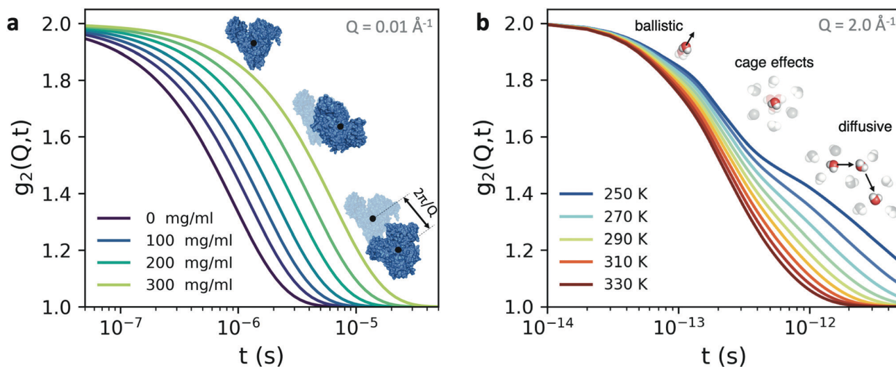
Fig. 3 The intensity autocorrelation function g_2(Q, t) calculated for (a) Bovine Serum Albumin (BSA) protein at Q = 0.01 \text{ \AA}^{-1} . The calculation utilizes the Stokes–Einstein relation and assumes diffusive behaviour and the different curves correspond to increasing protein concentration. By changing the Q range one can effectively probe different length scales of protein dynamics, as depicted in the inset. In this case, the dynamics take place from nanoseconds to microseconds. (b) The g_2(Q, t) of liquid and supercooled water estimated from the intermediate scattering function obtained by molecular dynamics. 62 Here, the momentum transfer Q = 2.0 \text{ \AA}^{-1} corresponds to atomic length scales and the correlation decay consists of three separate regimes: the early ballistic motion and the later diffusive regime. Between these two regimes appear cage effects, where molecules experience a transient confinement by their neighbors, which become increasingly pronounced upon supercooling.
