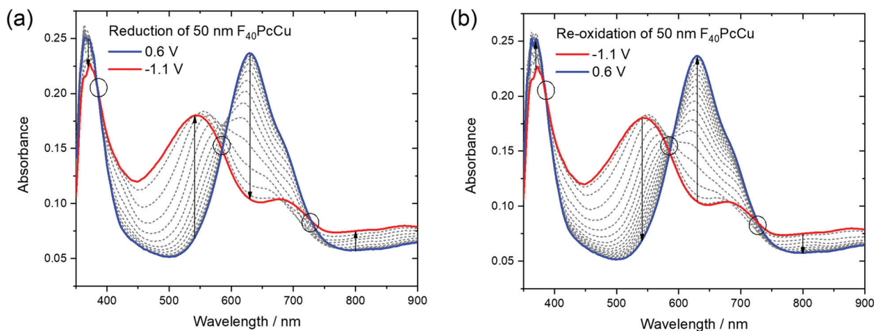
Fig. 9 Optical absorption spectra of a 50 nm thin film of F_{40}PcCu measured during cyclic voltammetry at 0.05\text{ V s}^{-1} upon (a) reduction and (b) re-oxidation of the film. The isosbestic points and ranges are marked by circles.
