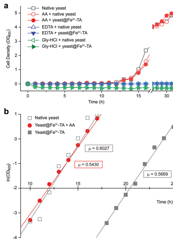
Fig. 3 (a) Growth curve of yeast@ \text{Fe}^{3+} -TA in the YPD broth (YPD_MPC[+]) with AA (100 mM, solid red circle), EDTA (100 mM, solid blue triangle), or gly-HCl (pH 2, solid green triangle). The data for native yeast incubated in the YPD broth (YPD_MPC[−]) with AA, EDTA, or gly-HCl are depicted as open symbols for each case and those for native yeast in the as-prepared YPD broth are depicted as open grey squares. (b) Linear-fitted plots from -4.0 to 1.0 of \ln(\text{OD}_{600}) of native yeast (open grey square), and yeast@ \text{Fe}^{3+} -TA incubated in the as-prepared YPD (solid grey square) or the AA-added YPD broth (solid red circle). The slope, \mu , is expressed in \ln units per hour, corresponding to the cell-growth rate in the exponential growth phase.
