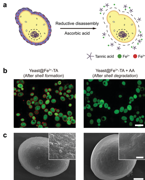
Fig. 2 (a) Schematic representation of the reduction-based \text{Fe}^{3+} -TA shell degradation on S. cerevisiae with ascorbic acid. (b) CLSM and (c) FE-SEM images of S. cerevisiae after shell formation and degradation. In (b), the \text{Fe}^{3+} -TA shell was stained with BSA-Alexa Fluor 647 (red) for shell visualization and S. cerevisiae was stained with FDA (green) for viability assay. Scale bar: 10 \mu\text{m} . In (c), scale bar: 1 \mu\text{m} , and 100 nm for the inset.
