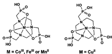
Scheme 4 Molecular structures of metalloligands \text{M}^{\text{III}}(\text{notpH}_3) and \text{M}^{\text{II}}(\text{notpH}_4) .
