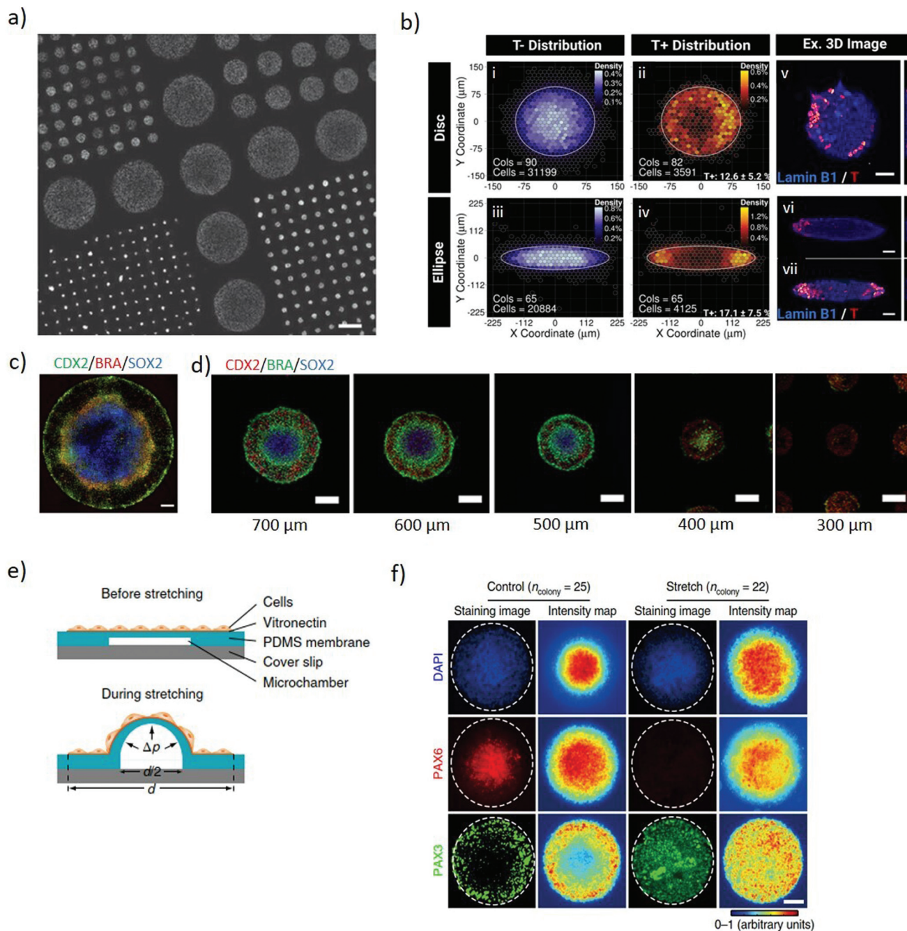
Fig. 2 Micropatterning stem cell colonies induces differential germ layer specification. (a) Glass coverslip coated with poly-D-lysine micropatterns of different diameters for selective hESC adhesion to the functionalised regions. Adapted with permission. 39 Copyright 2014, Nature Publishing Group. (b) The geometry of the micropatterned colonies influences the pattern of Brachyury (T) expression. T expression identifies the position a pre-streak like population. Binned density maps (BDMs) images (i–iv) and confocal images (v–vii) show that brachyury positive cells (T+, red) are positioned at the tips of the ellipse micropattern whilst in the disc micropatterns, T+ cells are located on the entire circumference. Cols = number of colonies analysed; cells = number of cells analysed. Scale bars = 50 \mu\text{m} . Adapted with permission. 41 Copyright 2018, The Company of Biologists Ltd. (c) Immunofluorescence of micropatterned hESC treated with BMP4, displaying radial organization of the trophectoderm (CDX2) and germ layers markers: mesoderm (BRA) and ectoderm (SOX2). Scale bars = 100 \mu\text{m} . Adapted with permission. 39 Copyright 2014, Nature Publishing Group. (d) Immunofluorescence images showing pattern-size dependence of germ-layer domains. As size is reduced SOX2 expression declines and eventually disappears. Scale bars = 200 \mu\text{m} . Adapted with permission. 32 Copyright 2017, The Company of Biologists Ltd. (e) Schematic of the micropatterned cell colonies on locally-stretchable PDMS membrane. The central region of the patterned colony stretches upon expansion of the underlying microfluidic channel. (f) Immunofluorescence images and average intensity maps of unstretched (control) and mechanically stretched (stretched) colonies at the central portion at day 8. Staining the colonies with Pax6 (neuroepithelial cell marker) and Pax3 (neural plate border marker), suggest that mechanical stimulation plays a role in regulating neural plate border differentiation. White dashed lines mark the colony periphery. Scale bar = 100 \mu\text{m} . (e and f) Adapted with permission. 42 Copyright 2018, Nature Publishing Group.
