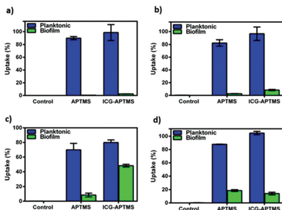
Fig. 5 Intracellular quantification of APTMS@SPIONs and ICG-APTMS@SPIONs in (a) E. coli , (b) K. pneumoniae , (c) P. aeruginosa and (d) S. epidermis . Samples at 425 \mu\text{g ml}^{-1} Fe concentration were incubated with bacteria for 24 h. Intracellular Fe amounts were determined by ICP-MS.
