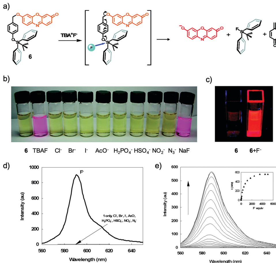
Fig. 5 Sensing mechanism and performance of 6 . (a) Reaction scheme of 6 with TBAF. (b) Color changes of 6 (5 \mu M) in \text{CH}_3\text{CN}/\text{H}_2\text{O} (50 : 50, v/v) after the addition of 3000 equiv. various anions. (c) Solution of 6 before and after addition of \text{F}^- under a UV lamp (365 nm). (d) Comparison of the fluorescence emission spectra of 6 (0.5 \mu M) in acetonitrile after the addition of 1400 equiv. of various anions. (e) Fluorescence titration of 6 (5 \mu M) upon the addition of TBAF in \text{CH}_3\text{CN}/\text{H}_2\text{O} (50 : 50, v/v). Inset: Emission intensity change of 6 upon the addition of \text{F}^- at 589 nm. Reproduced with permission from ref. 20. Copyright 2007, American Chemical Society.
