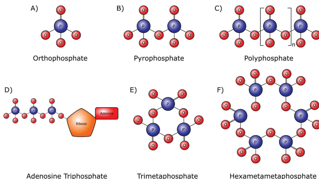
Fig. 2 Chemical structures of linear and cyclic inorganic phosphate structures with varying chain lengths. (A) Orthophosphate (Pi). (B) Pyrophosphate (PPi). (C) Inorganic polyphosphate (polyP). (D) Adenosine triphosphate (ATP). (E) Trimetaphosphate (TMP). (F) Hexametaphosphate (HMP).
