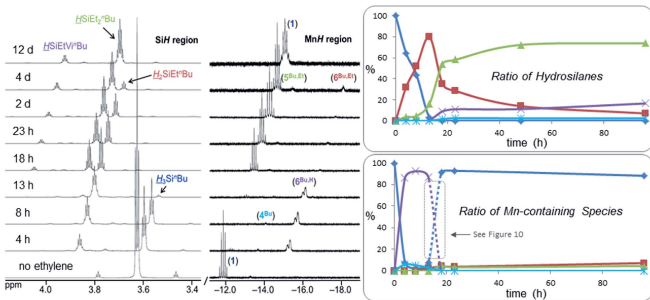
Fig. 9 \text{SiH} (left) and \text{MnH} (middle) regions of the ^1\text{H} NMR spectra (298 K, 500 or 600 MHz) for the hydrosilylation of ethylene by \text{H}_3\text{Si}^n\text{Bu} using [(\text{dmpe})_2\text{MnH}(\text{C}_2\text{H}_4)] ( 1 ) pre-catalyst (7 mol% relative to the hydrosilane) under \sim 1.7 atm of ethylene (initial, n_{\text{C}_2\text{H}_4} \approx 40 \times n_{\text{silane}} ) in \text{C}_6\text{D}_6 and after various time intervals at 60^\circ\text{C} . The x-axis corresponds to the bottom ^1\text{H} NMR spectrum, and for clarity, each spectrum above that is shifted by 0.3 ( \text{SiH} region) or 0.4 ( \text{MnH} region) ppm to lower frequency. Right: graphs showing the ratio of (top) hydrosilanes (dark blue \blacklozenge = \text{H}_3\text{Si}^n\text{Bu} ; red \blacksquare = \text{H}_2\text{SiEt}^n\text{Bu} ; green \blacktriangle = \text{HSiEt}_2^n\text{Bu} ; purple \times = \text{HSiEtVi}^n\text{Bu} ; light blue * = unidentified \text{SiH} -containing silane) and (bottom) \text{MnH} -containing species {dark blue \blacklozenge = [(\text{dmpe})_2\text{MnH}(\text{C}_2\text{H}_4)] ( 1 ); light blue * = [(\text{dmpe})_2\text{MnH}(\text{SiH}_2^n\text{Bu})_2] ( 4^{\text{Bu}} ); green \blacktriangle = [(\text{dmpe})_2\text{MnH}_2(\text{SiHEt}^n\text{Bu})] ( 5^{\text{Bu,Et}} ); purple \times = [(\text{dmpe})_2\text{MnH}^n\text{BuHSi}=\text{CHMe}] ( 6^{\text{Bu,H}} ); red \blacksquare = [(\text{dmpe})_2\text{MnH}^n\text{BuEtSi}=\text{CHMe}] ( 6^{\text{Bu,Et}} ) in these reactions, as measured by ^1\text{H} NMR spectroscopy. Reaction details can be found in the ESI pg. S15.†
